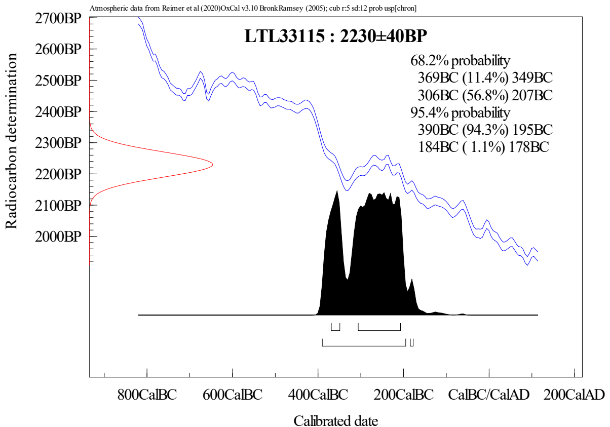
Figure 1. Calibration of the radiocarbon age of the sample LTL33115.
