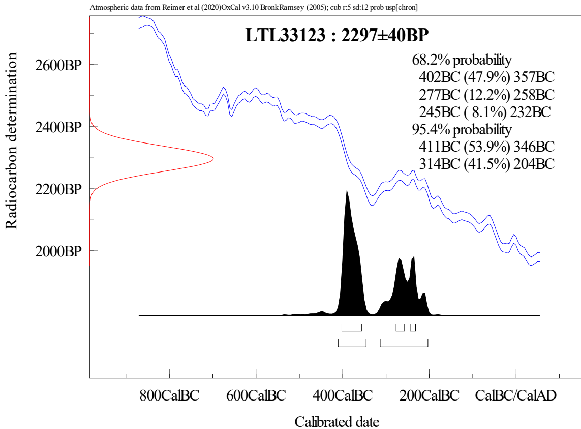
Figure 1. Calibration of the radiocarbon age of the sample LTL33123.
