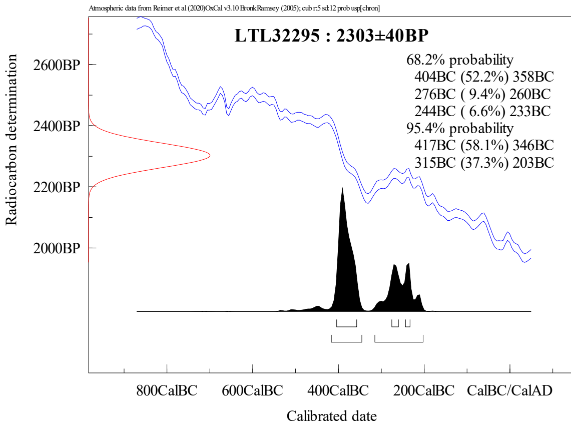
Figure 1. Calibration of the radiocarbon age of the sample LTL32295.
